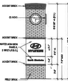
08 - ENLARGED ELEVATION SCALE 1/8" = 1'-0"
